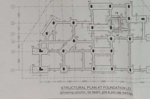
STRUCTURAL PLAN AT FOUNDATION LEVEL (Showing columns, beams, pile caps & pile cap markings)
